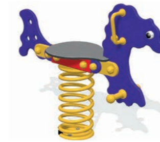
DRAGON CODE: A1314 W 3000mm x D 3000mm Free Fall Height: <600mm
