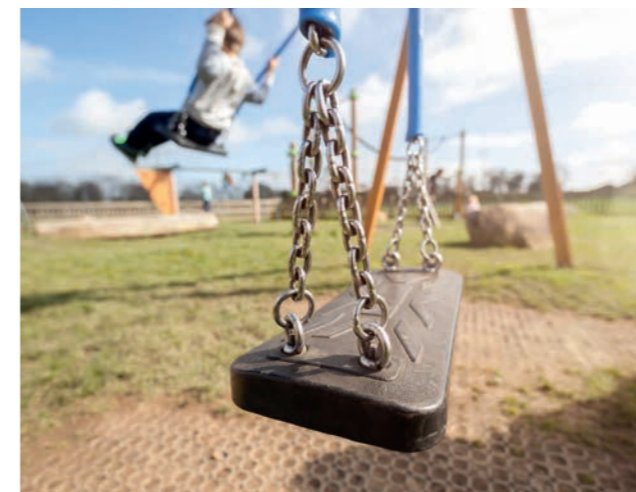
DOUBLE SWING CODE: A1060 W 8000mm x D 4000mm Free Fall Height: 1500mm
